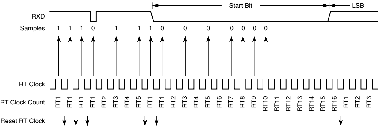
Figure 10-22. Start Bit Search Example 1
