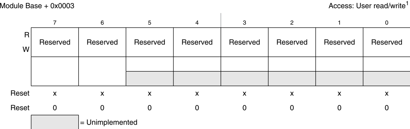
Figure 14-5. Reserved Register
