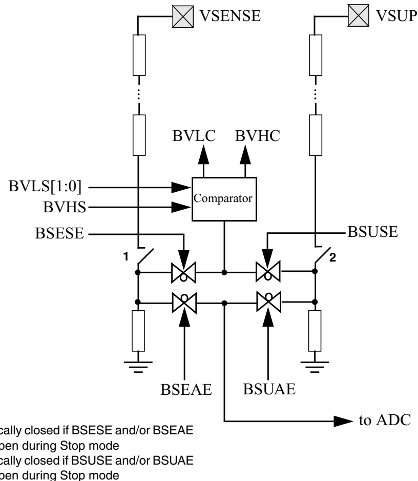
Figure 16-1. BATS Block Diagram
