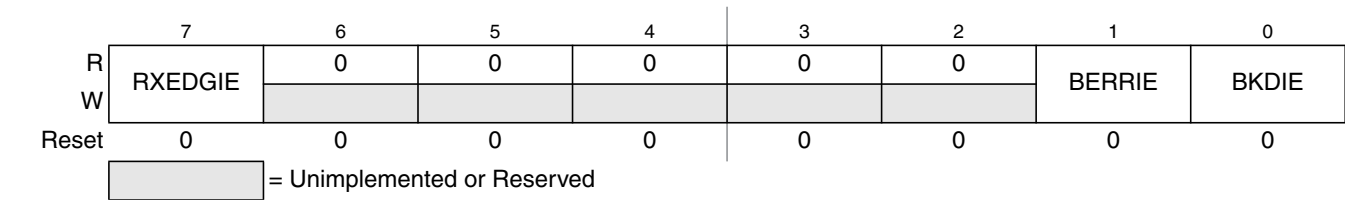
Figure 10-7. SCI Alternative Control Register 1 (SCIACR1)
