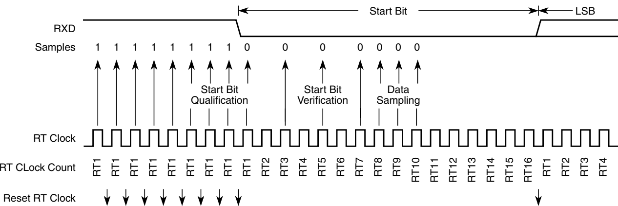
Figure 10-21. Receiver Data Sampling
