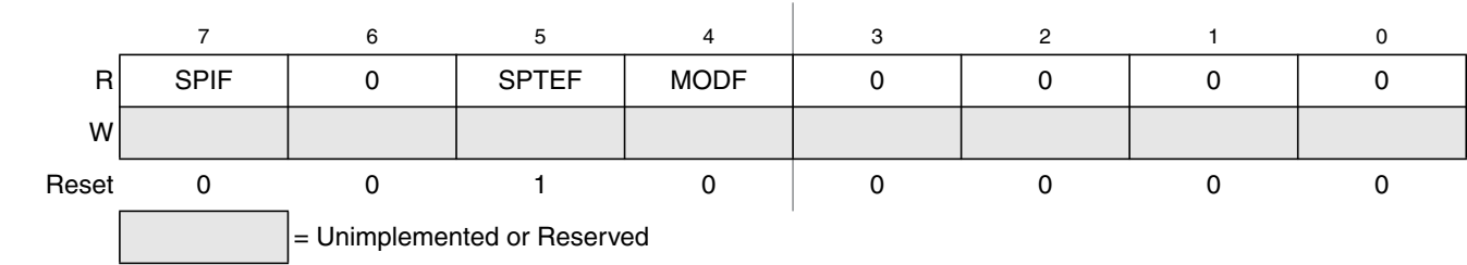
Figure 11-6. SPI Status Register (SPISR)
