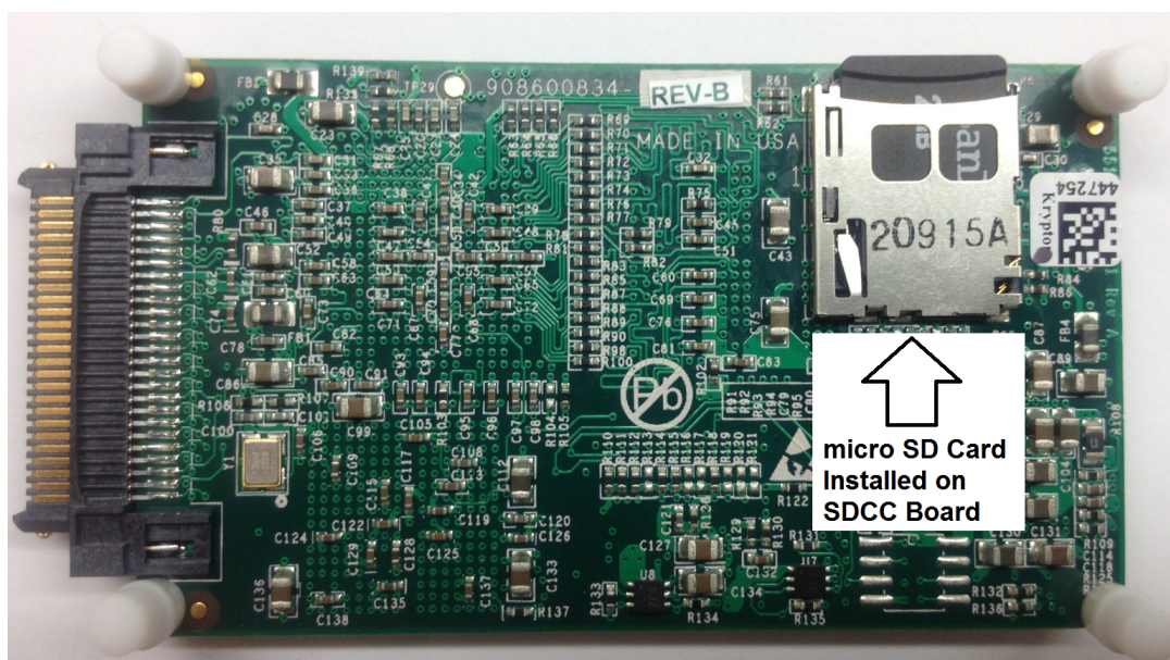
Figure 5. Bottom View of SDCC Board with microSD Memory Card Installed
