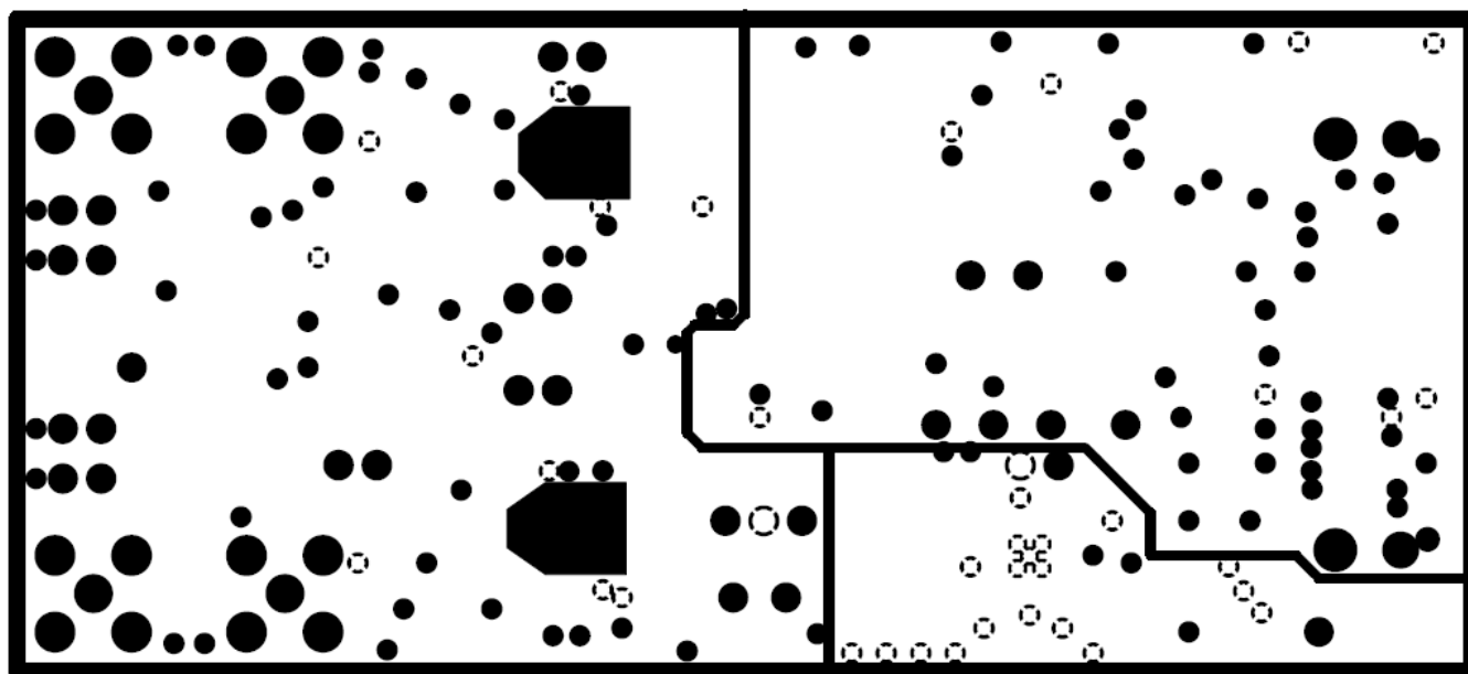
Figure 27. ADS7851EVM PCB: Power Layer
