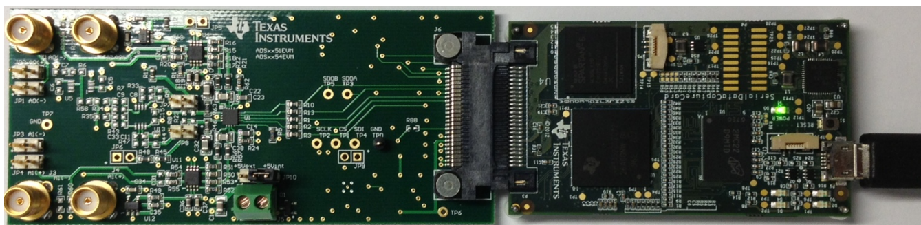
ADS7851EVM-PDK
