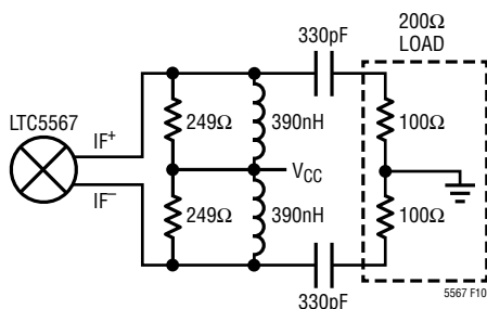
Figure 10. Wideband 200 \Omega Differential Output
