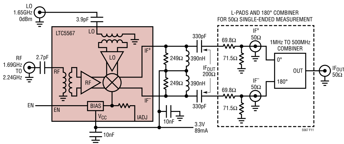
Figure 11. Test Circuit for Wideband 200 \Omega Differential Output
