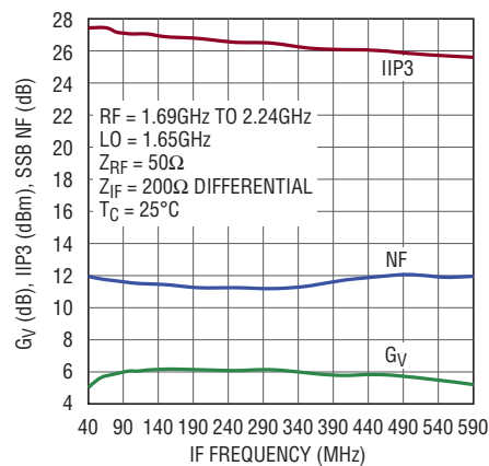
Figure 12. Voltage Conversion Gain, IIP3 and NF vs IF Output Frequency for Wideband 200 \Omega Differential IF
