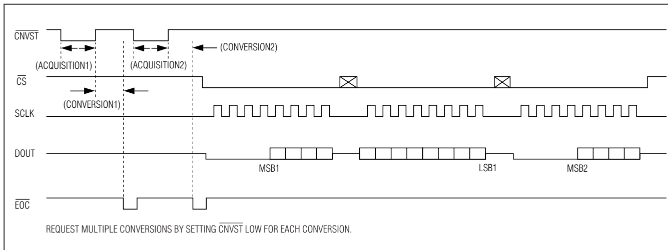
Figure 5. Clock Mode 01
