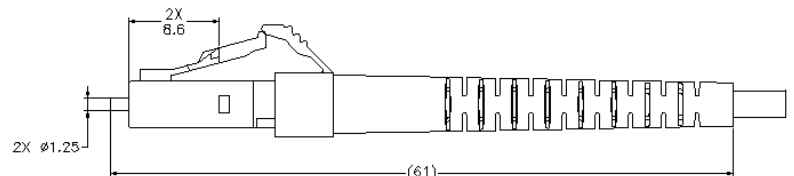
LC Duplex Connector with Flex Boot
