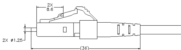
with 1.6/2.0mm Short Boot
