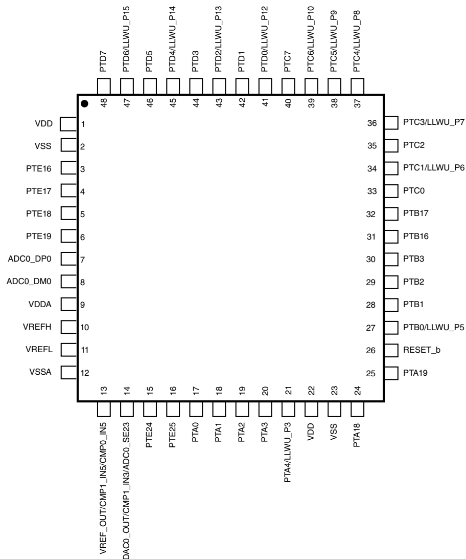
Figure 24. K02F 48 LQFP pinout diagram
