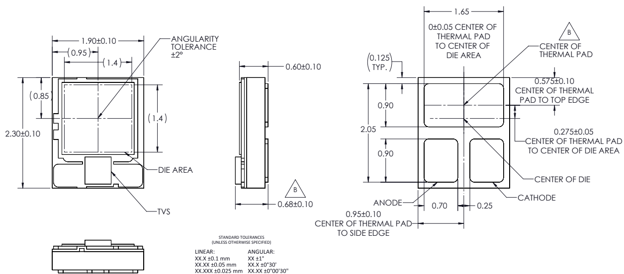
Figure 10. Mechanical dimensions for LUXEON F ES Cool White.
