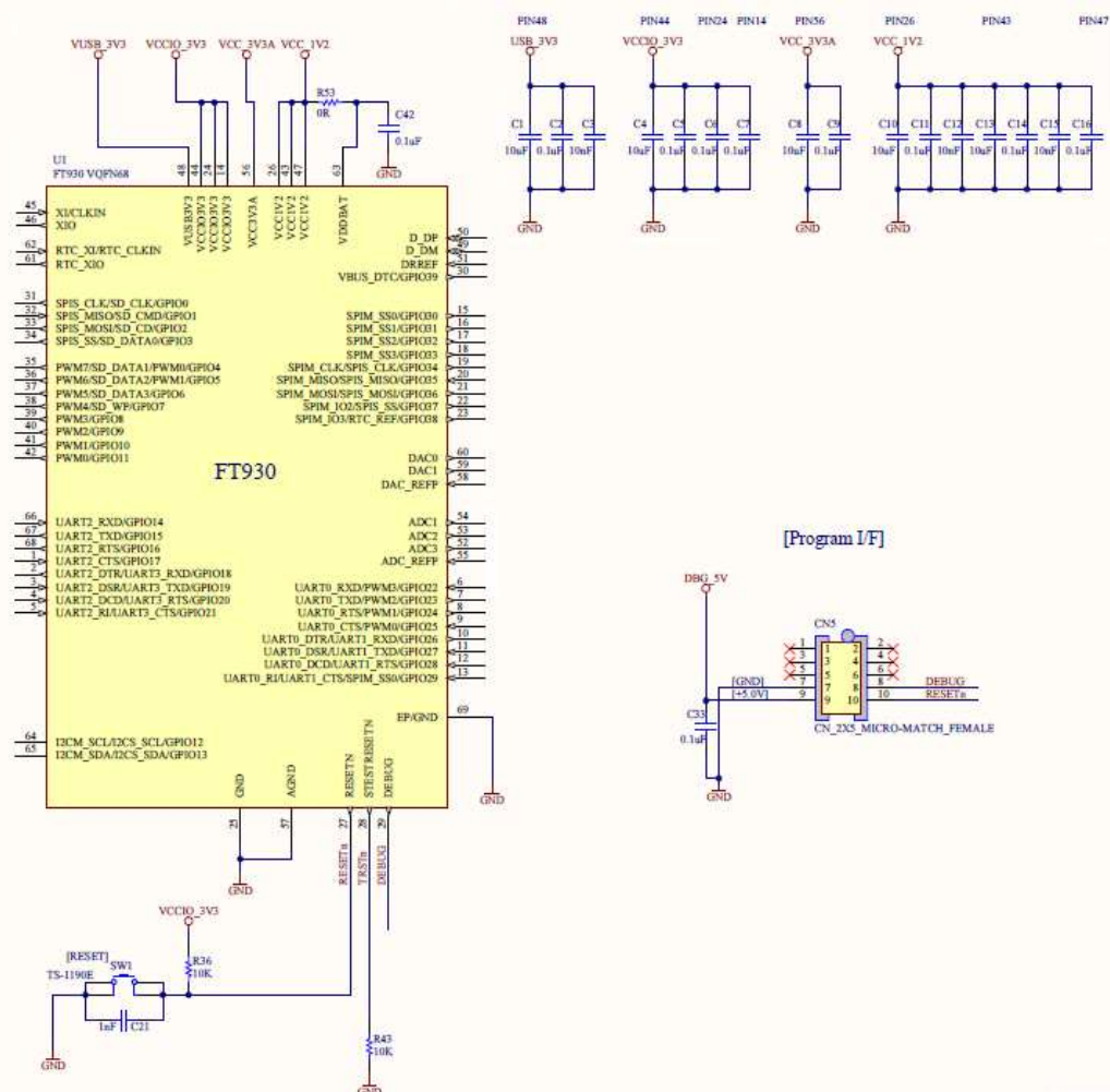
Figure 4-6 – Programmer Interface
