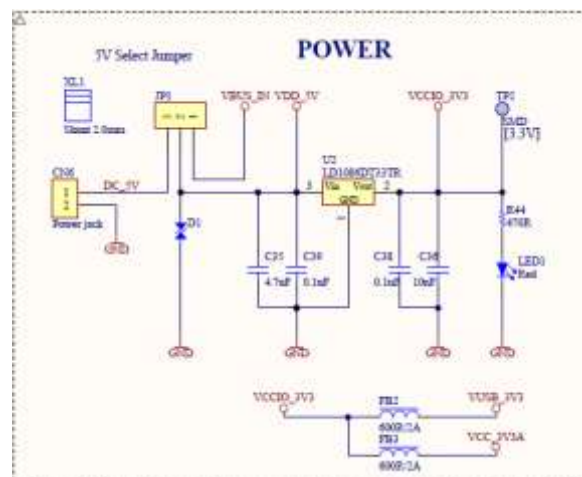
Figure 4-2– Power supply
