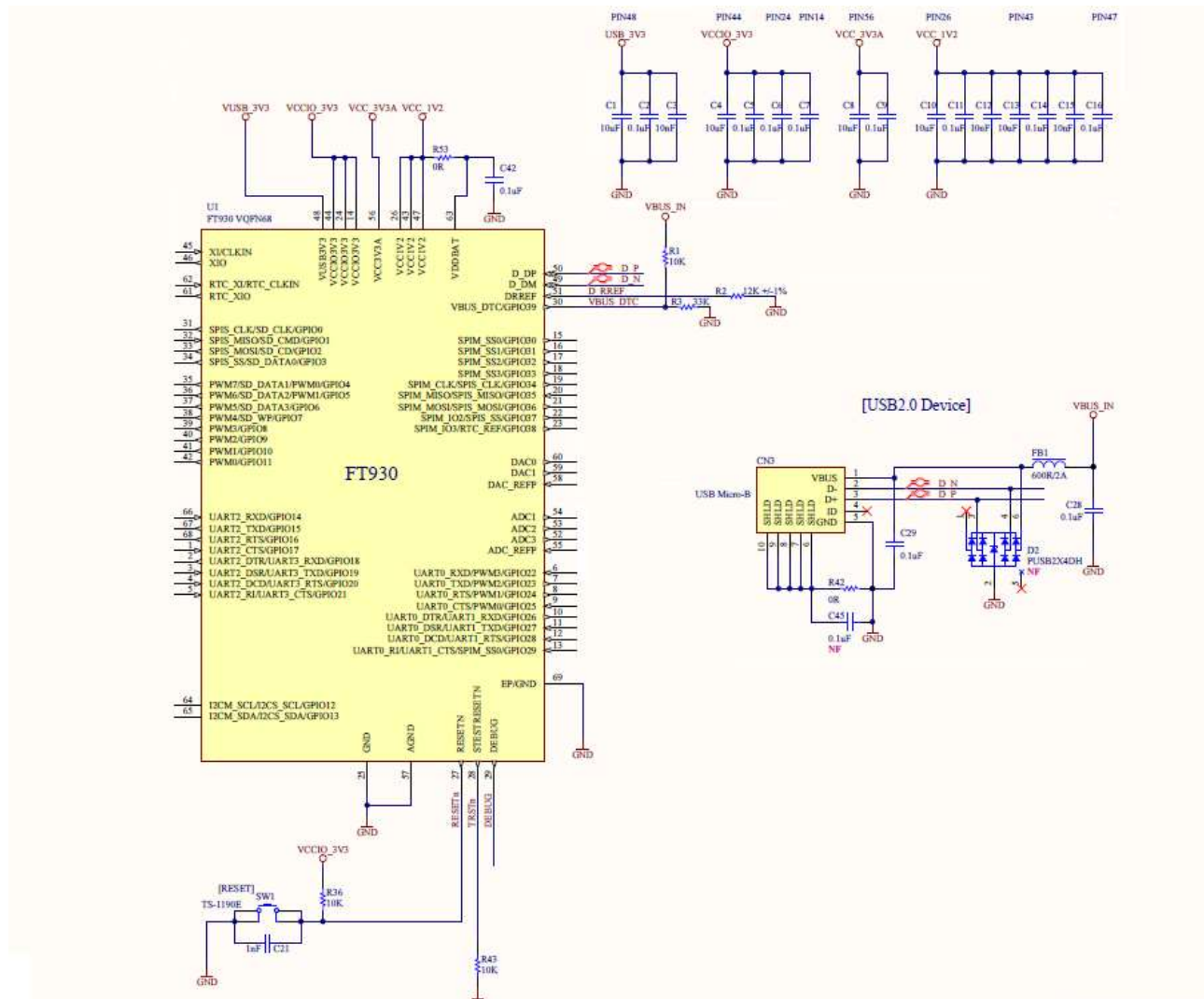
Figure 4-5- USB Connectors
