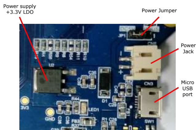
Figure 4-2– Power supply
