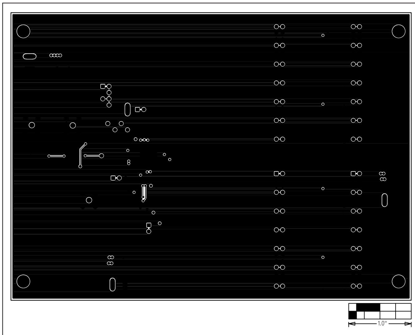
Figure 6. MAX1213/MAX1214/MAX1215 EV Kit PC Board Layout—Solder Side
