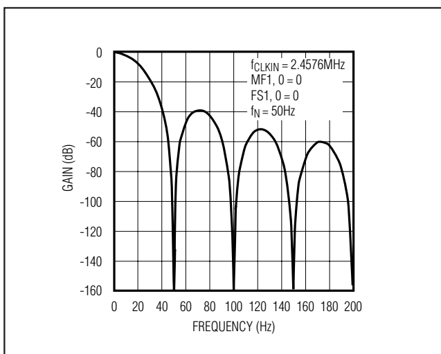
Figure 11. Frequency Response of the SINC 3 Filter (Notch at 50Hz)
