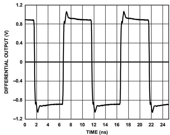
Figure 17. LVPECL Output (Differential) @ 100 MHz
