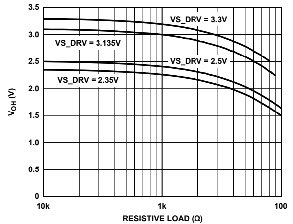
Figure 16. CMOS Output V_{OH} (Static) vs. R_{LOAD} (to Ground)
