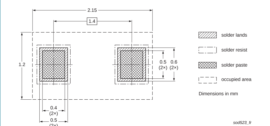
Fig 30. Reflow soldering footprint BAS516 (SOD523/SC-79)
