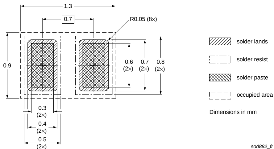
Fig 21. Reflow soldering footprint BAS16L (SOD882/DFN1006-2)
