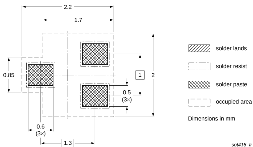
Fig 22. Reflow soldering footprint BAS16T (SOT416/SC-75)
