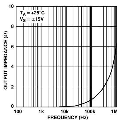
TPC 9. Closed-Loop Output Impedance vs. Frequency
