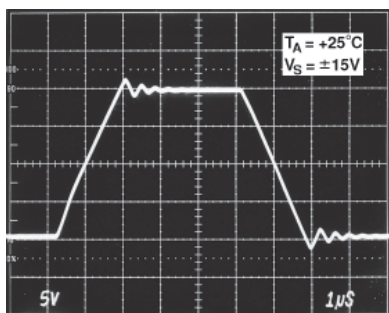
TPC 4. Large Signal Transient Response
