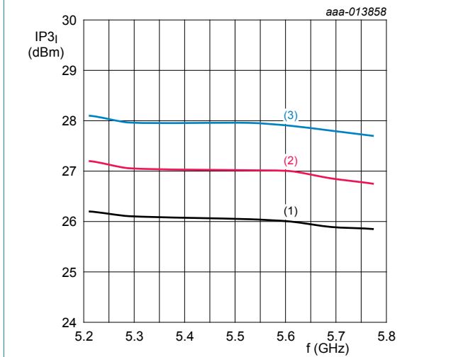
Figure 28. Input third-order intercept point as a function of frequency at different supply voltages
