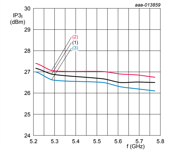
Figure 29. Input third-order intercept point as a function of frequency at different ambient temperatures
