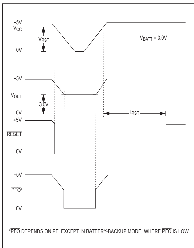
Figure 2. Timing Diagram
