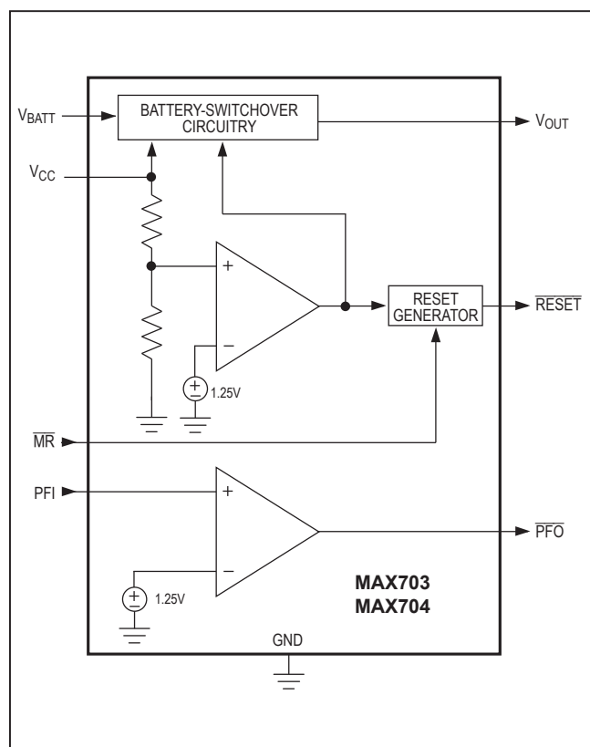
Figure 1. Block Diagram
