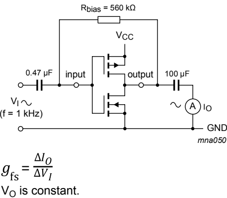
Fig. 9. Test set-up for measuring forward transconductance
