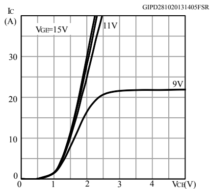
Figure 5. Output characteristics ( T_J = 25^\circ C )
