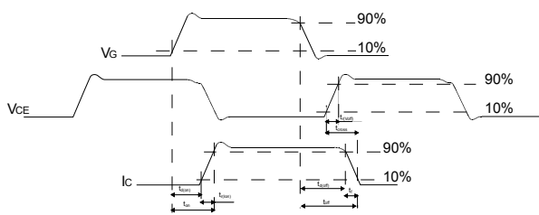
Figure 34. Switching waveform
