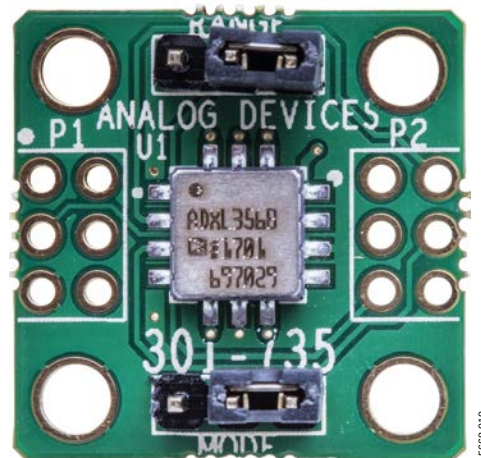
Figure 1. EVAL-ADXL356BZ/EVAL-ADXL356CZ
