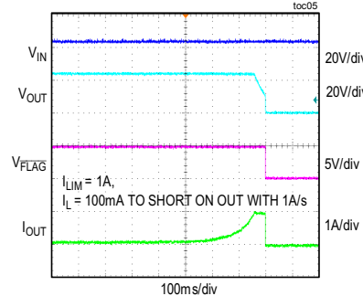
CURRENT-LIMIT RESPONSE
