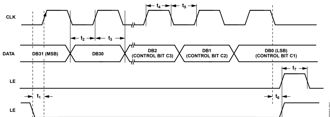
Figure 2. Timing Diagram
