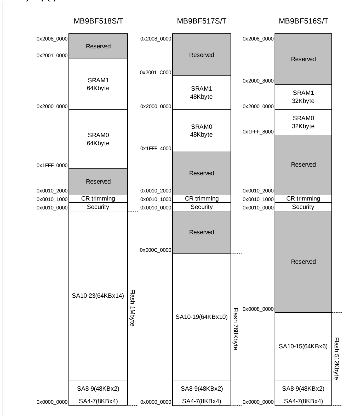
Memory Map (2)
