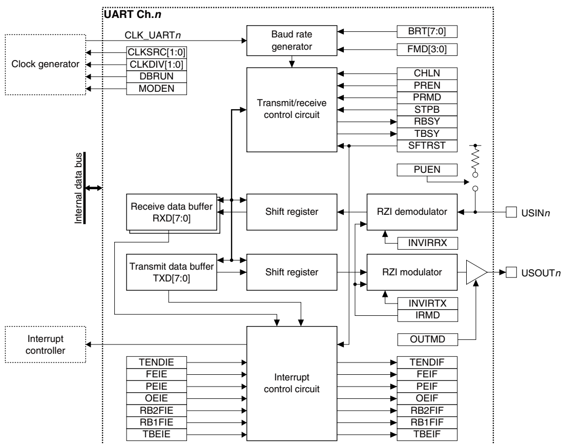
Figure 11.1.1 UART Configuration
