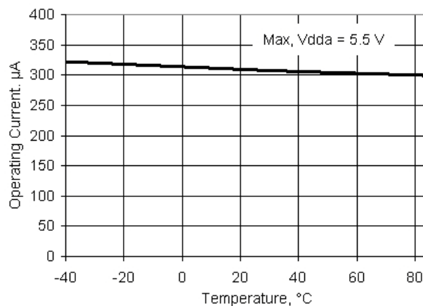
Figure 11-54. VDAC Operating Current vs Temperature, 1 V Mode, Fast Mode
