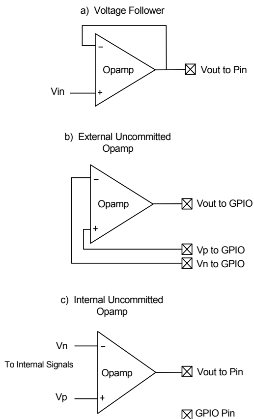
Figure 8-8. Opamp Configurations
