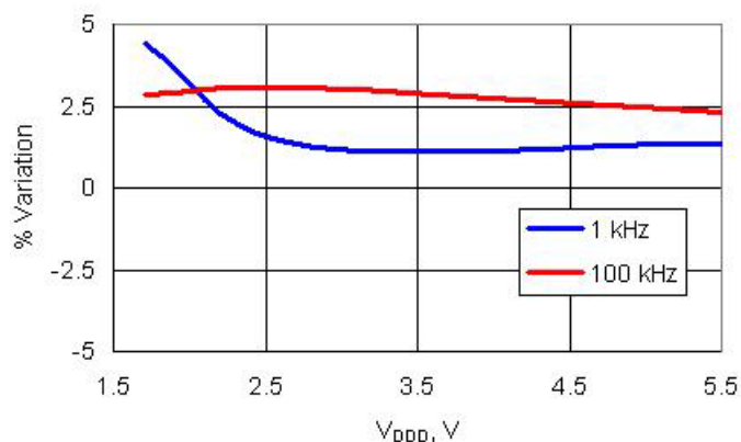
Figure 11-72. ILO Frequency Variation vs. V_{DD}
