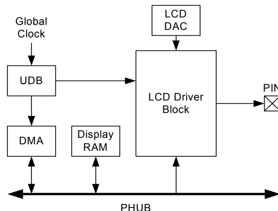
Figure 8-11. LCD System
