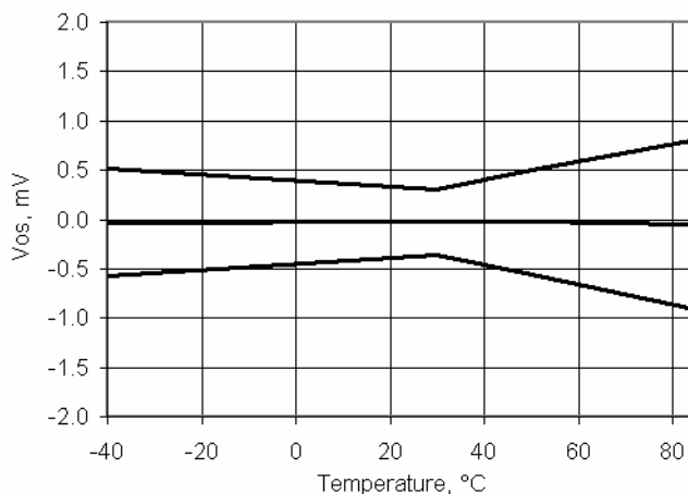
Figure 11-26. Opamp Voffset vs Temperature, Vdda = 5 V
