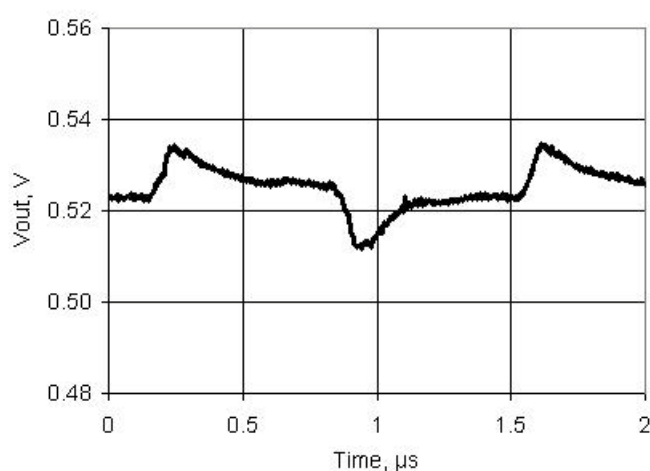
Figure 11-56. VDAC Glitch Response, Codes 0x7F - 0x80, 1 V Mode, Fast Mode, Vdda = 5 V
