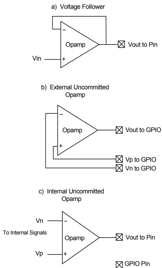
Figure 8-8. Opamp Configurations
