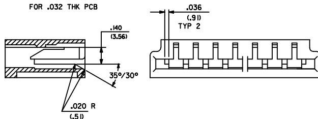
OPTION CODE E FOR .032 THK PCB
