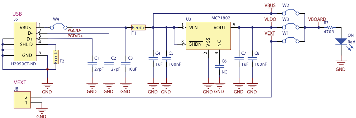
Figure 7. Power Supply Schematic
