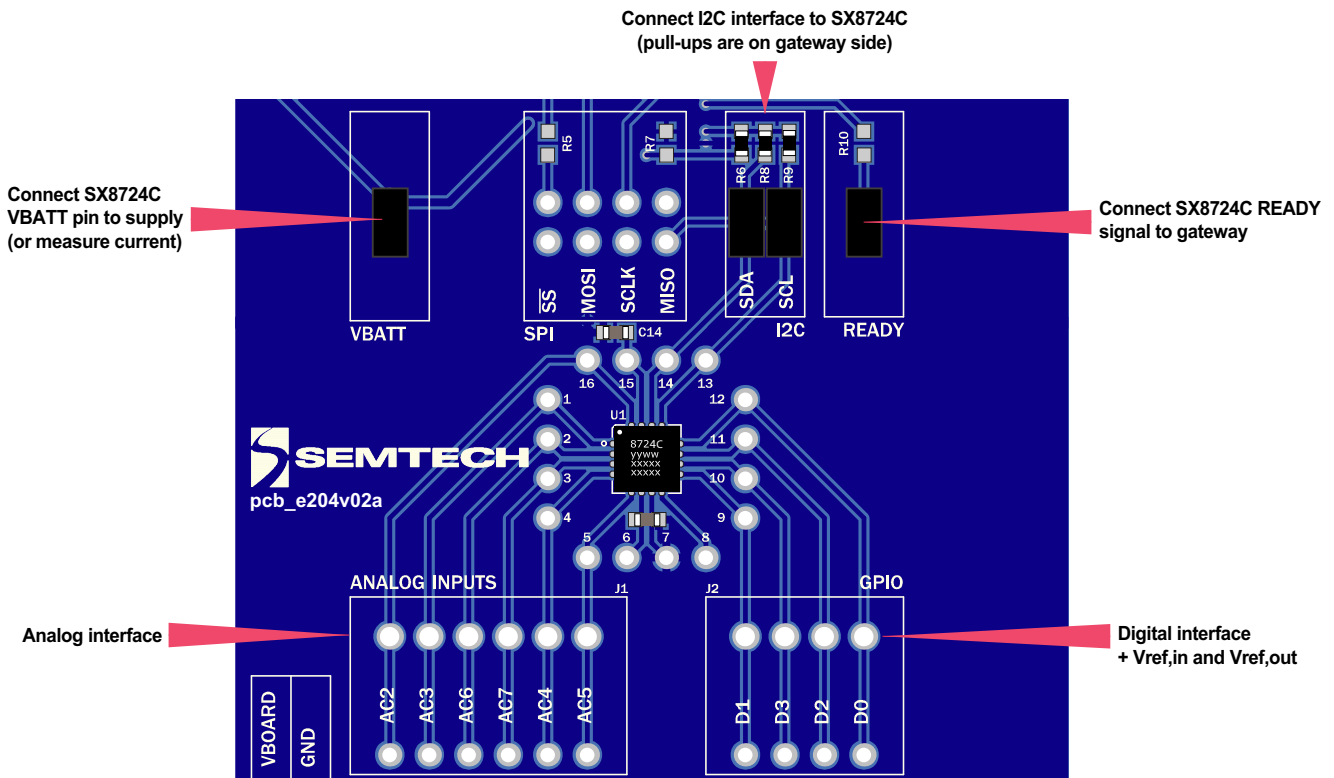
Figure 5. SX8724C Interface on the Board
