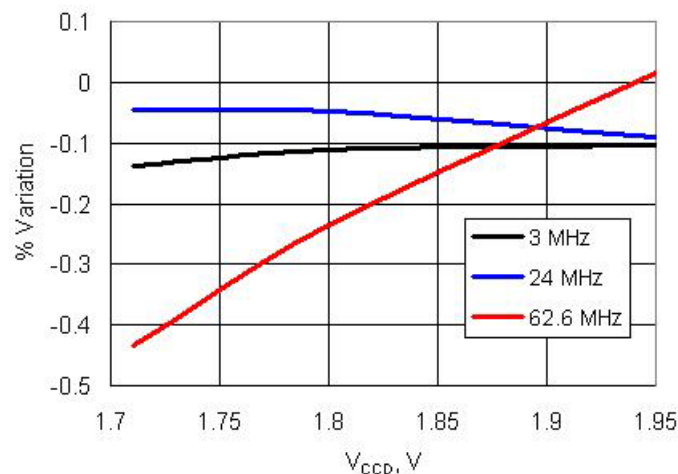
Figure 11-70. IMO Frequency Variation vs. V_{CC}
