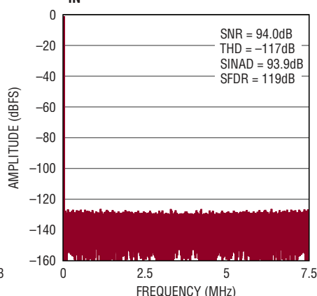
32k Point FFT f_{\text{SAMPL}} = 15\text{Mpsps} , f_{\text{IN}} = 2\text{kHz}
