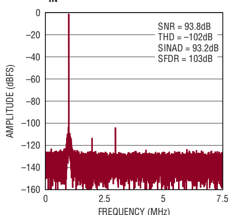
32k Point FFT f_{\text{SAMPL}} = 15\text{Mpsps} , f_{\text{IN}} = 1\text{MHz}
