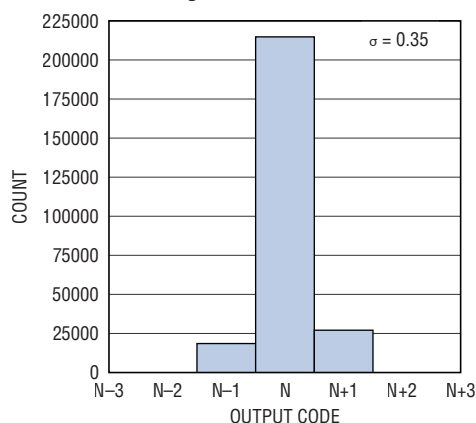
DC Histogram
