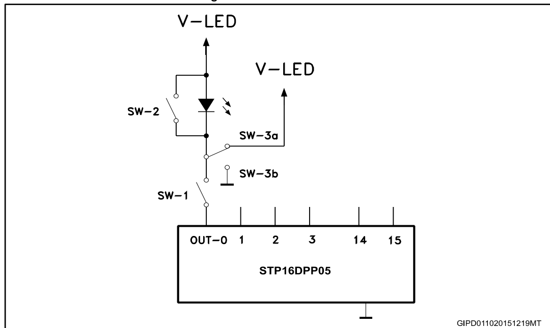
Figure 21: Detection circuit
