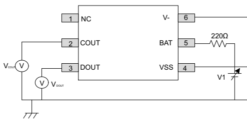
Figure 20. Test Circuit 1
