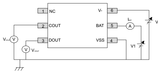
Figure 21. Test Circuit 2
