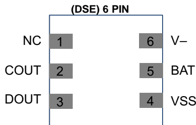
Pin Functions
