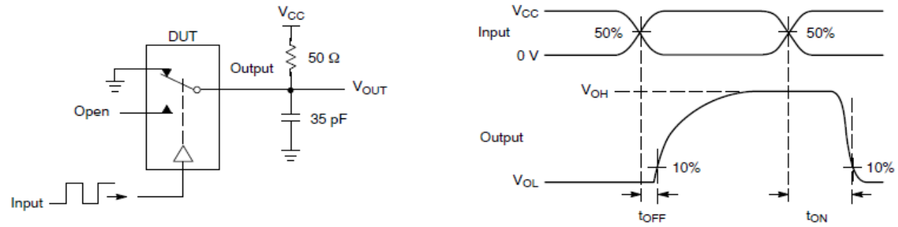
Figure 8. t_{ON} / t_{OFF}
