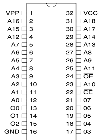
32-lead PDIP Top view
