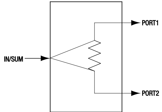
Figure 1. SKY16406-381LF Block Diagram
