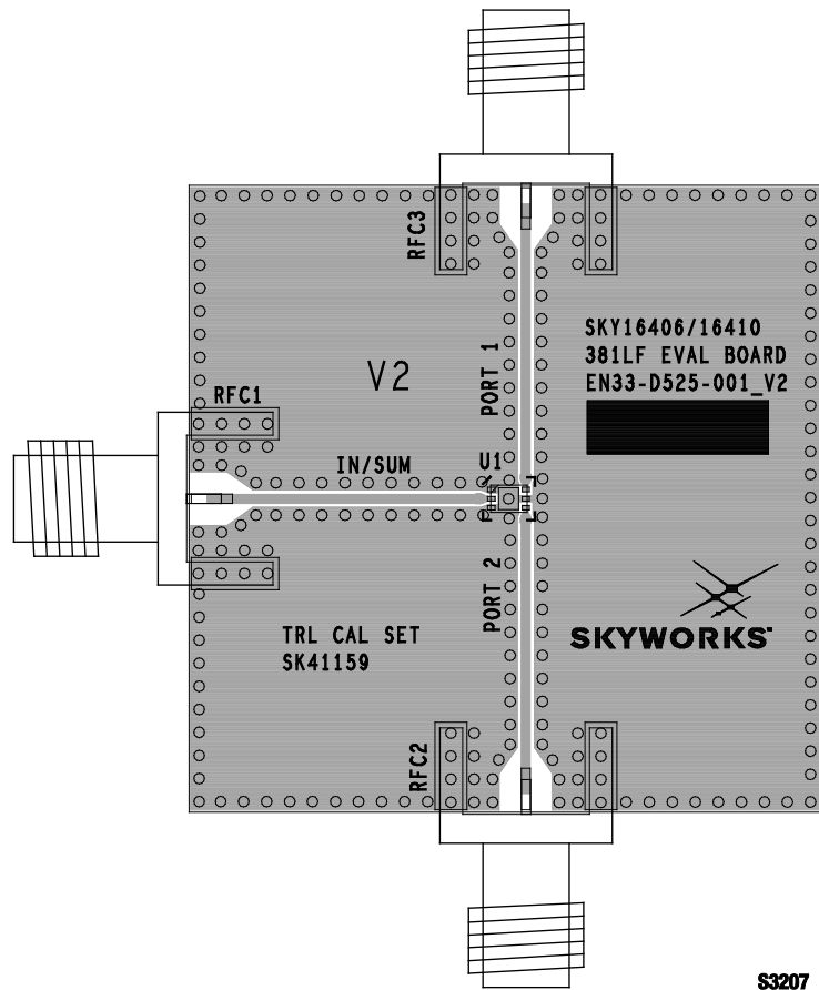
Figure 10. SKY16406-381LF Evaluation Board Assembly Diagram
