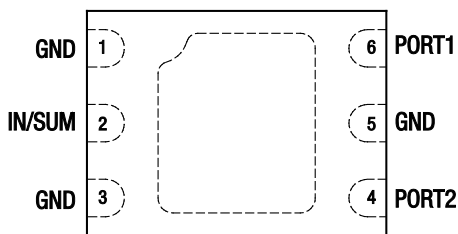
Figure 2. SKY16406-381LF Pinout – 6-Pin DFN (Top View)
