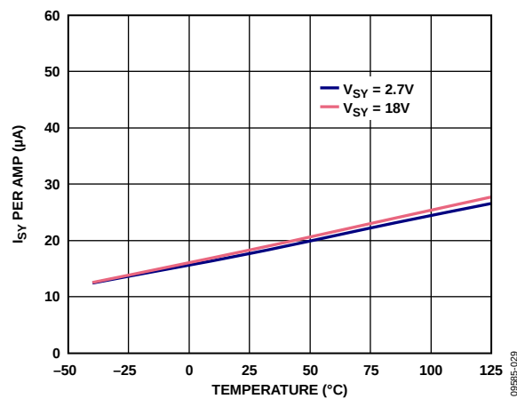
Figure 26. Supply Current per Amplifier vs. Temperature
