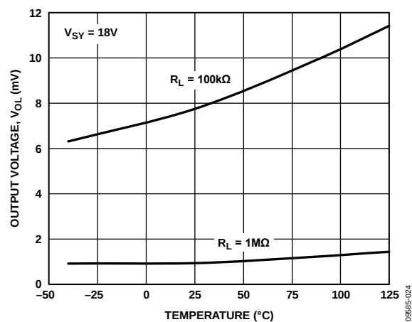
Figure 24. Output Voltage ( V_O ) vs. Temperature
