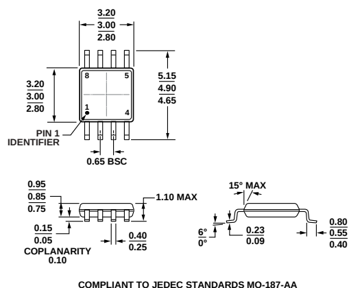
Figure 72. 8-Lead Mini Small Outline Package [MSOP] (RM-8)
