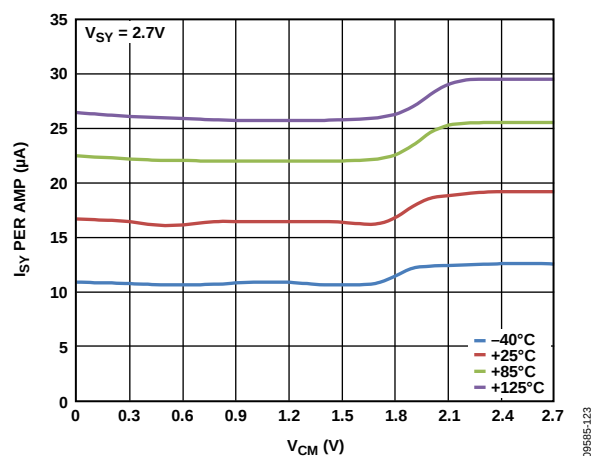
Figure 22. Supply Current per Amplifier vs. Common-Mode Voltage
