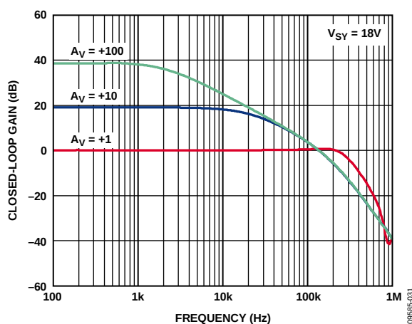
Figure 31. Closed-Loop Gain vs. Frequency
