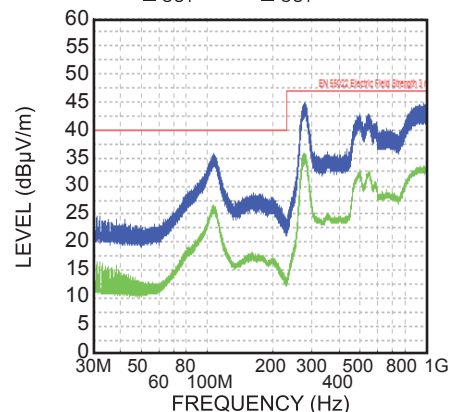
Radiated EMI
