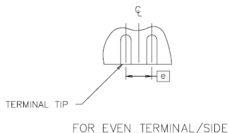
Figure 23. ZM7300 Terminals
