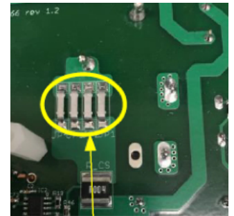
Remove jumpers and add a cable for inductor current measurement
