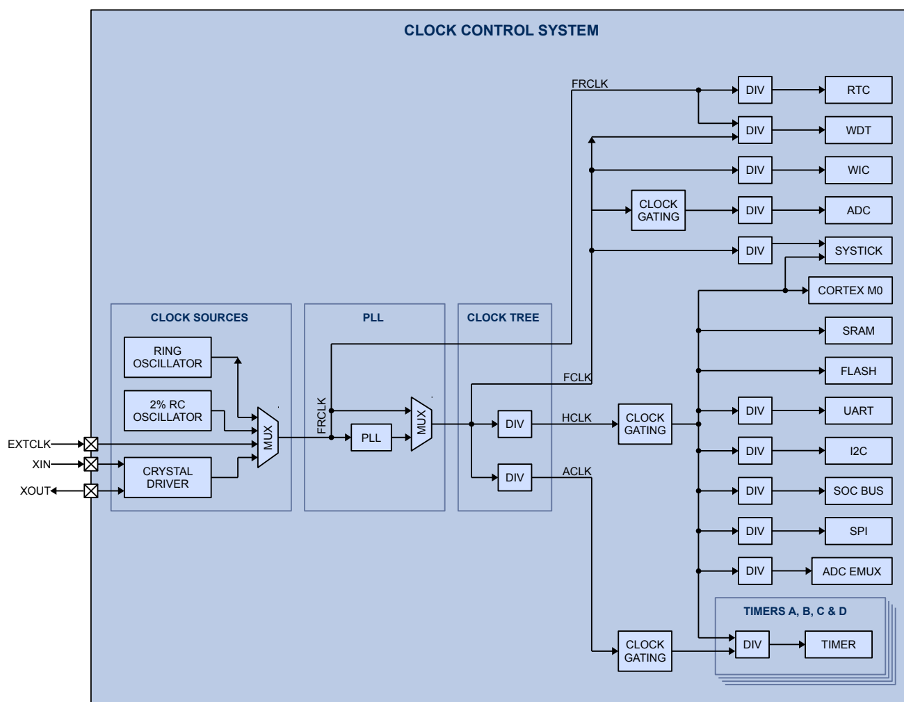
Figure 15-1 Clock Control System
