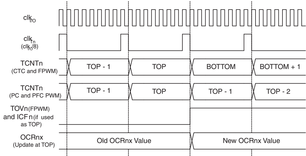
Figure 4-49. Timer/Counter Timing Diagram, with Prescaler ( f_{\text{clk\_I/O}}/8 )
