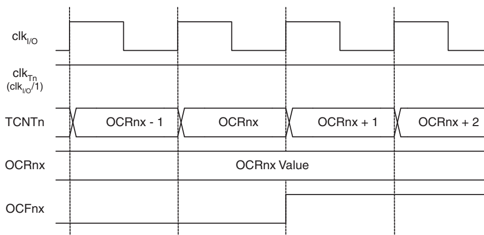
Figure 4-46. Timer/Counter Timing Diagram, Setting of OCF1x, no Prescaling
