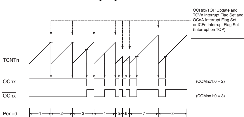
Figure 4-43. Fast PWM Mode, Timing Diagram
