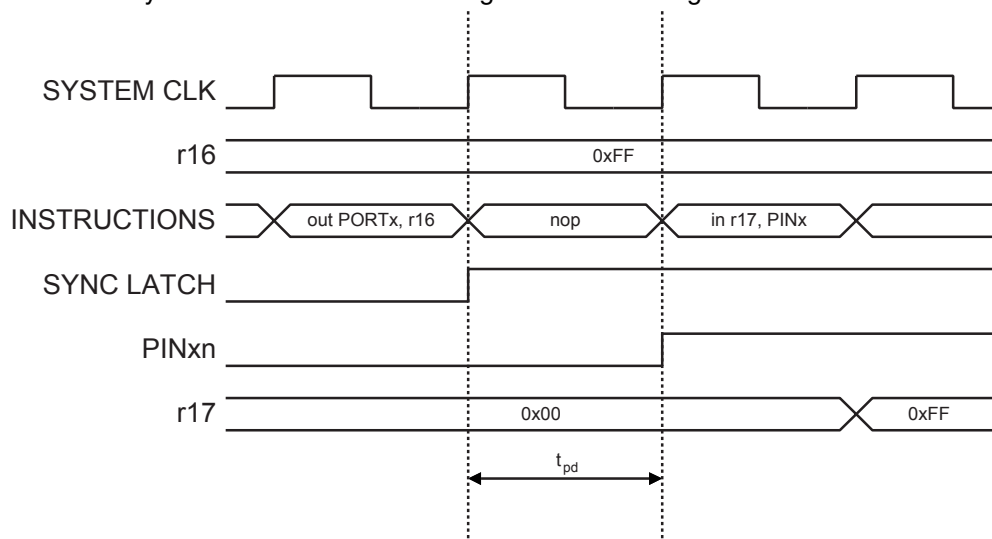
Figure 4-24. Synchronization when Reading a Software Assigned Pin Value
