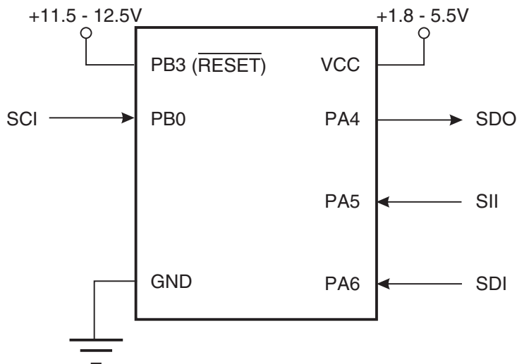
Figure 4-75. High-voltage Serial Programming
