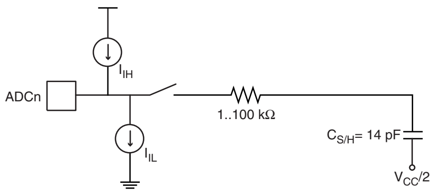
Figure 4-66. Analog Input Circuitry
