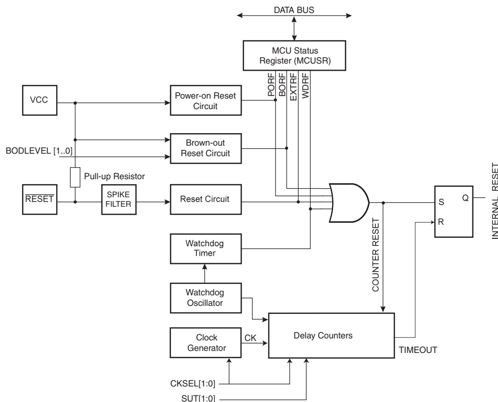
Figure 4-13. Reset Logic
