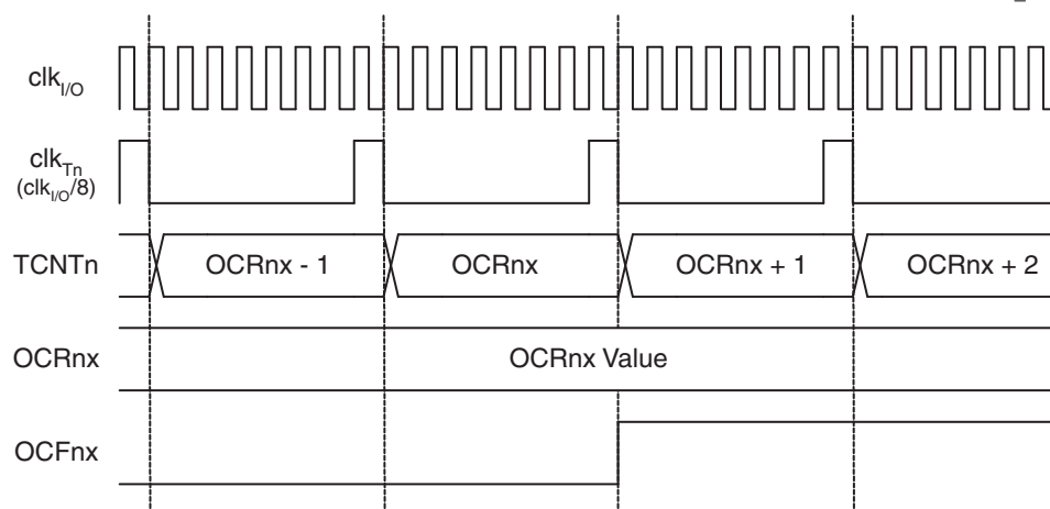
Figure 4-47. Timer/Counter Timing Diagram, Setting of OCF1x, with Prescaler ( f_{\text{clk}_{I/O}}/8 )
