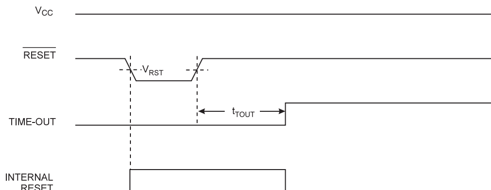
Figure 4-16. External Reset During Operation
