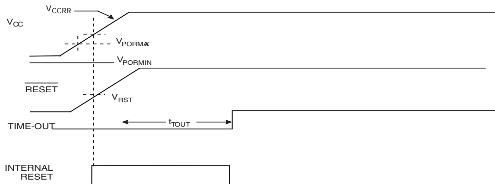
Figure 4-14. MCU Start-up, \overline{\text{RESET}} Tied to V_{CC}
