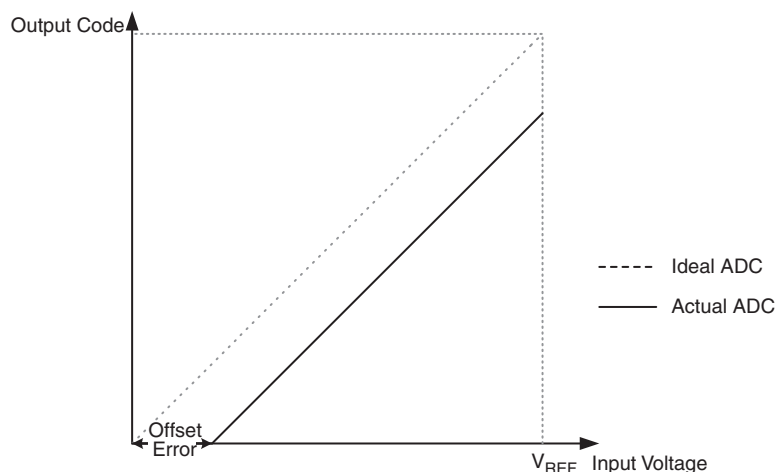
Figure 4-67. Offset Error
