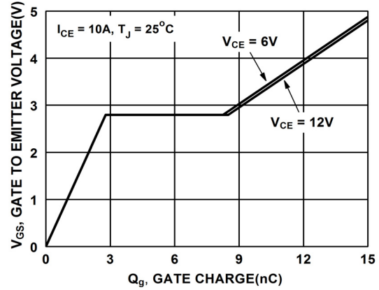
Figure 14. Gate Charge
