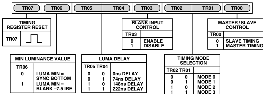
Figure 66. Timing Register 0
