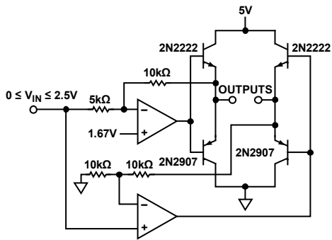
Figure 21. H Bridge
