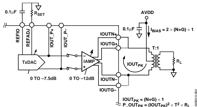
Figure 64. Current-Mode Operation
